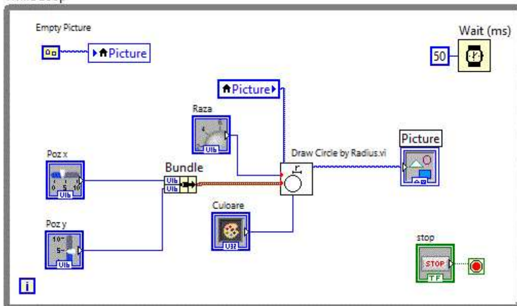
While Loop
